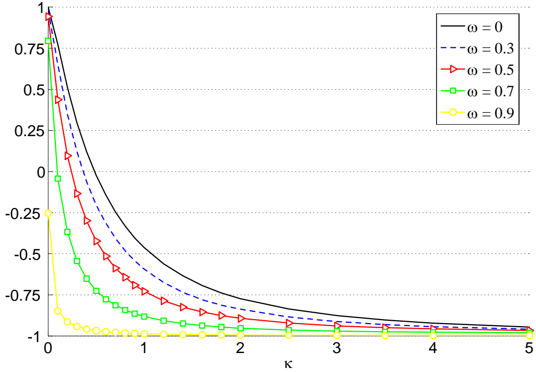
Figure 7: Interest-Output Correlation As a Function of \kappa , A Two-Sector Model (no demand shocks)*
