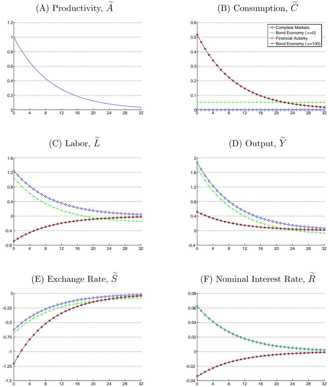
Figure 3: Impulse Response Functions 1 Percent Increase in Productivity
